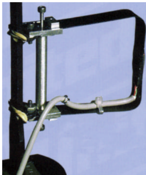
CO-2.0-2: High Elongation Clip-on Extensometer
